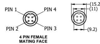
VIEW A
